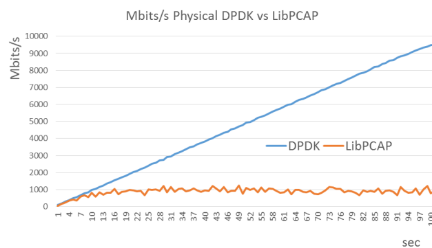
Figure 3-10 Physical Testbed DPDK vs LibPcap.
