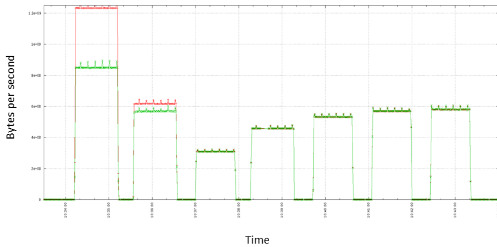
Figure 3-17 Throughput calculation for Docker container deployment.
