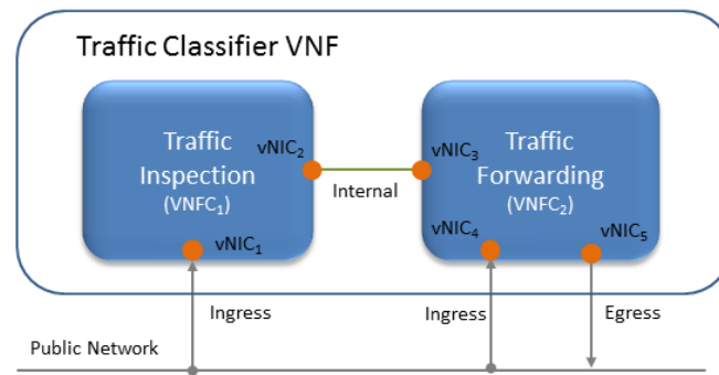
Figure 7-1 Virtualised Traffic Classifier High Level Architecture
